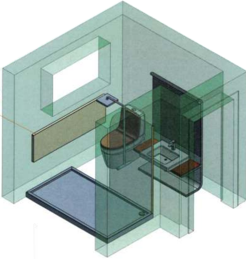
ECOLEC RADIANT PANEL HEATER DEPICTED ON BATHROOM WALL BATHROOM NOM. BATHROOM SIZE 2000 x 1700 ECOLEC PANEL SIZE 500 x 1500
